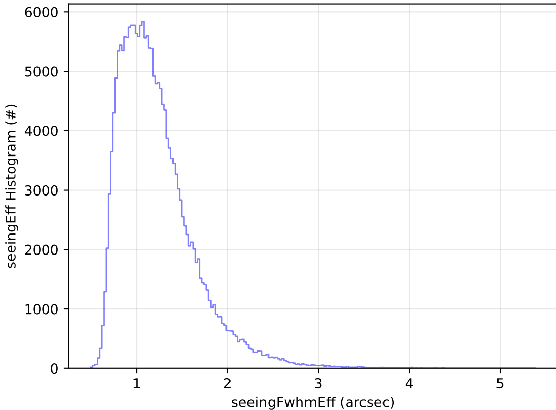
too_elab_r128_d2_griz_v3.4_10yrs All sky g band: seeingEff Histogram
