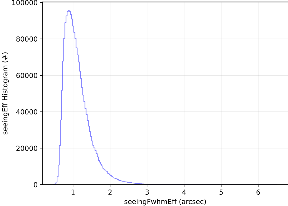
too_elab_r128_d2_griz_v3.4_10yrs All sky all bands: seeingEff Histogram
