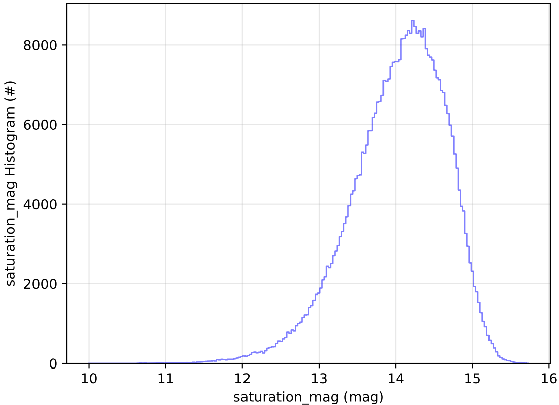
too_elab_r128_d2_griz_v3.4_10yrs WFD z band: saturation_mag Histogram
