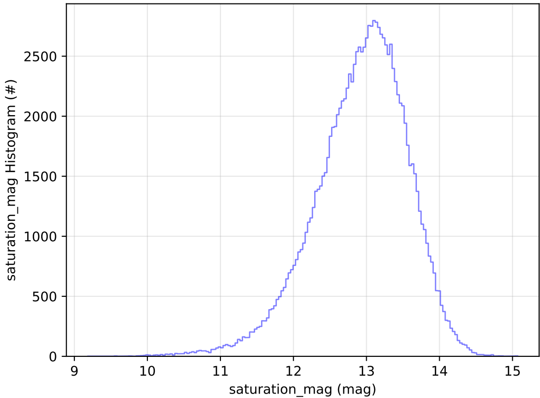
too_elab_r128_d2_griz_v3.4_10yrs WFD u band: saturation_mag Histogram
