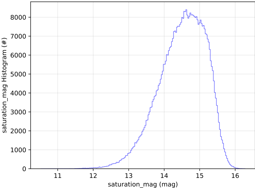
too_elab_r128_d2_griz_v3.4_10yrs WFD r band: saturation_mag Histogram
