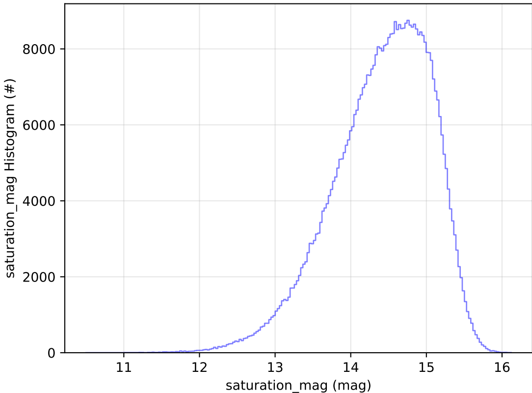
too_elab_r128_d2_griz_v3.4_10yrs WFD i band: saturation_mag Histogram
