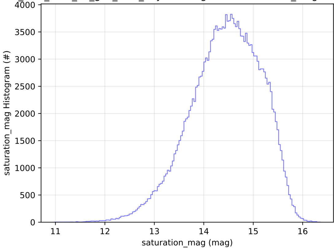
too_elab_r128_d2_griz_v3.4_10yrs WFD g band: saturation_mag Histogram
