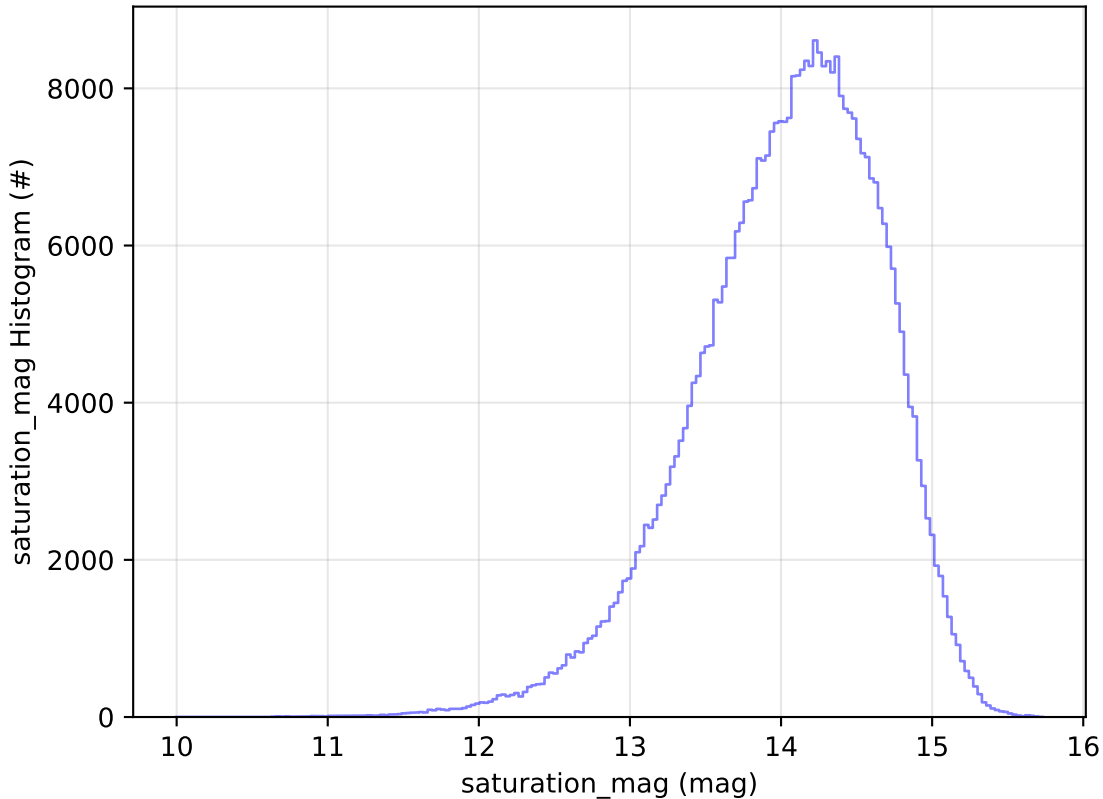
too_elab_r128_d2_griz_v3.4_10yrs All sky z band: saturation_mag Histogram
