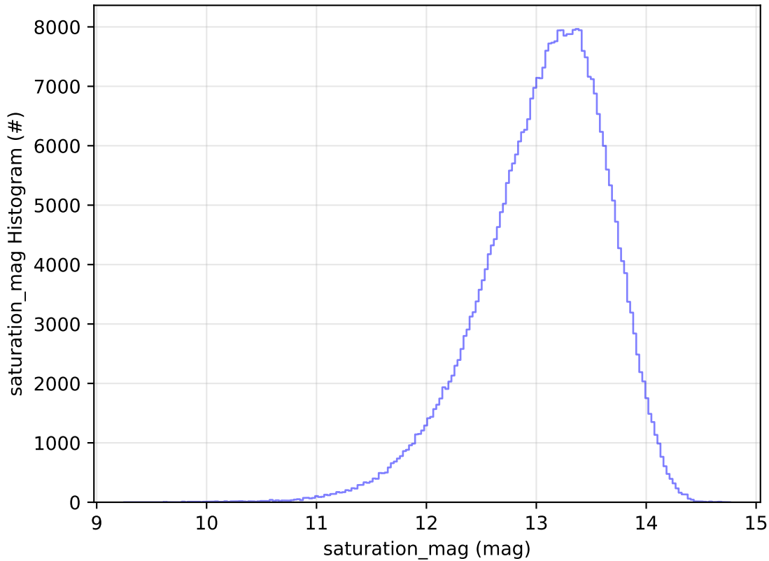
too_elab_r128_d2_griz_v3.4_10yrs All sky y band: saturation_mag Histogram
