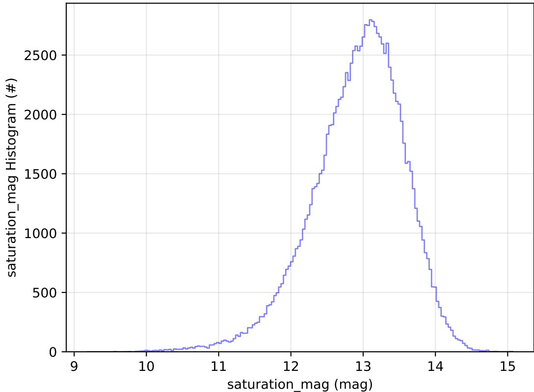
too_elab_r128_d2_griz_v3.4_10yrs All sky u band: saturation_mag Histogram
