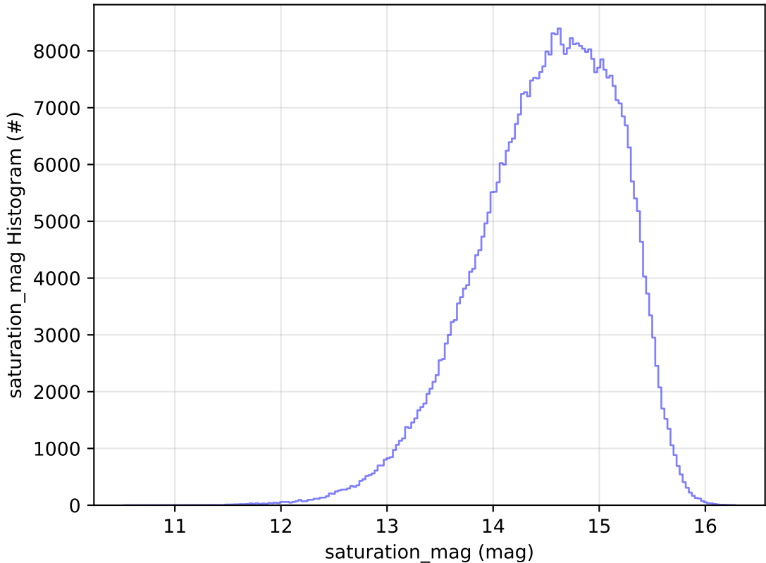
too_elab_r128_d2_griz_v3.4_10yrs All sky r band: saturation_mag Histogram
