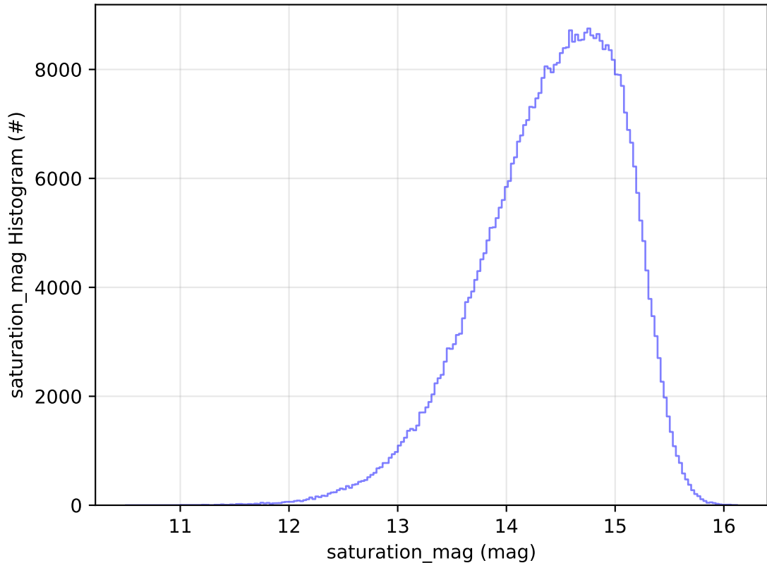
too_elab_r128_d2_griz_v3.4_10yrs All sky i band: saturation_mag Histogram
