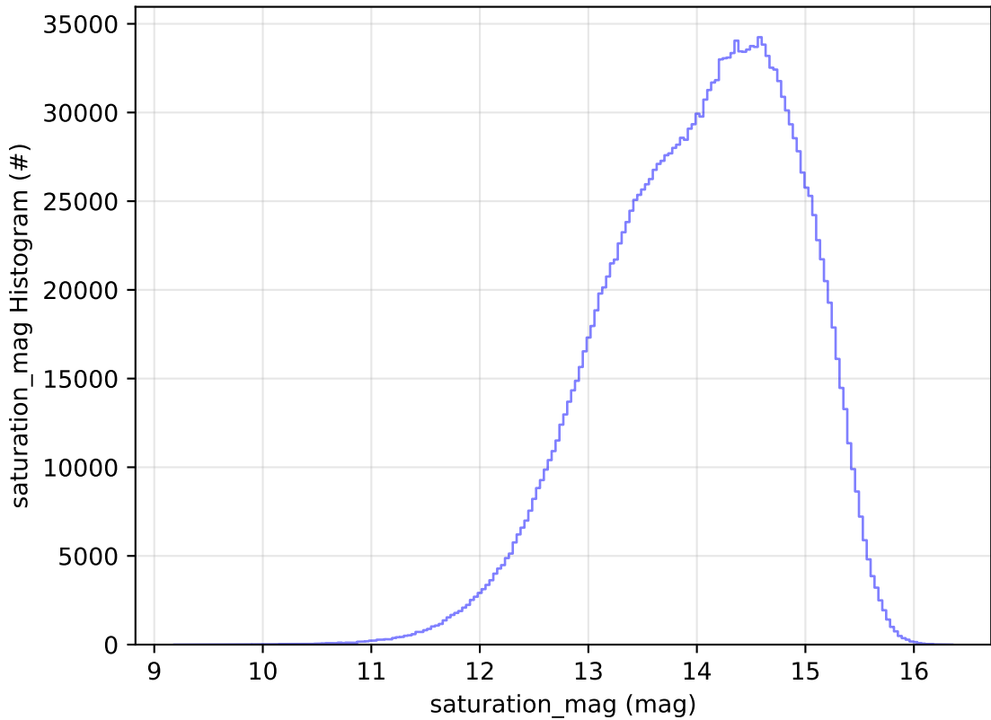
too_elab_r128_d2_griz_v3.4_10yrs All sky all bands: saturation_mag Histogram
