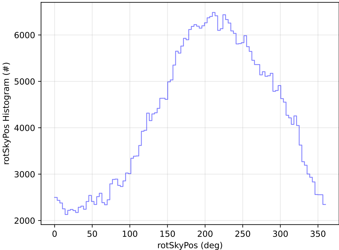
too_elab_r128_d2_griz_v3.4_10yrs WFD z band: rotSkyPos Histogram
