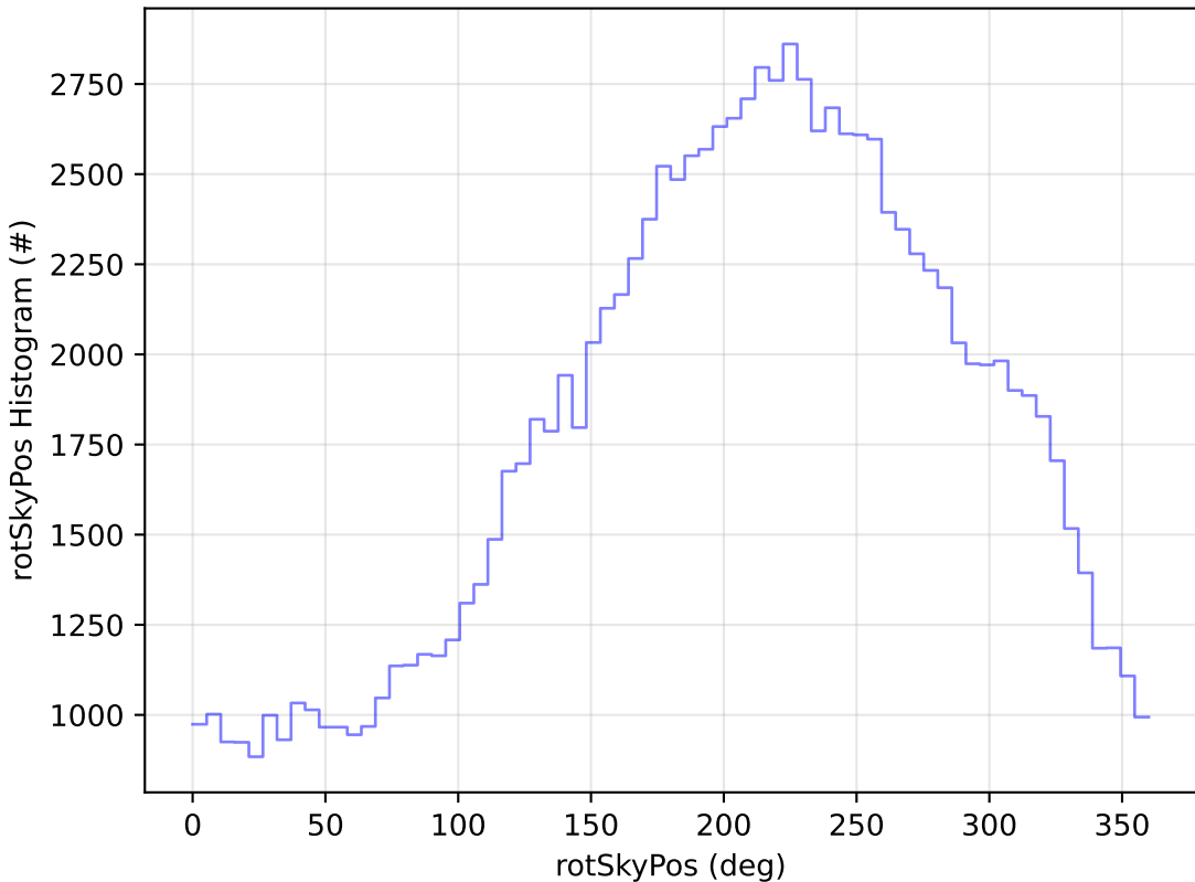
too_elab_r128_d2_griz_v3.4_10yrs WFD u band: rotSkyPos Histogram
