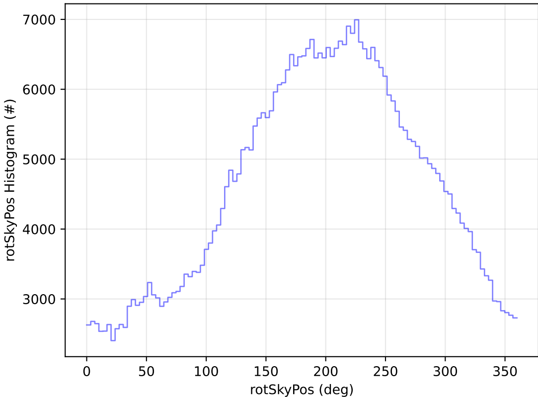
too_elab_r128_d2_griz_v3.4_10yrs WFD r band: rotSkyPos Histogram
