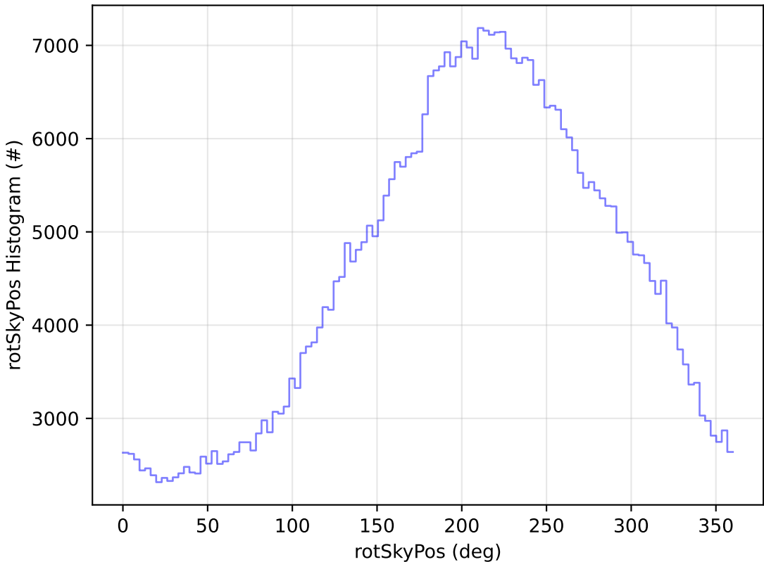
too_elab_r128_d2_griz_v3.4_10yrs WFD i band: rotSkyPos Histogram
