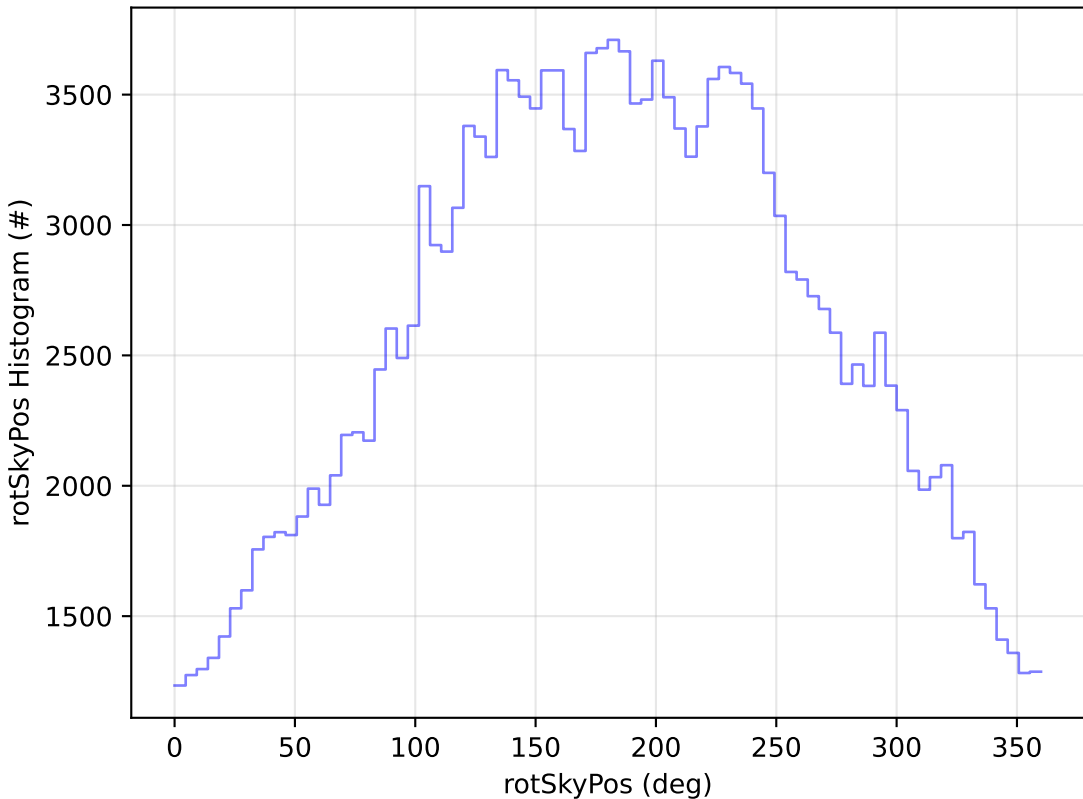
too_elab_r128_d2_griz_v3.4_10yrs WFD g band: rotSkyPos Histogram
