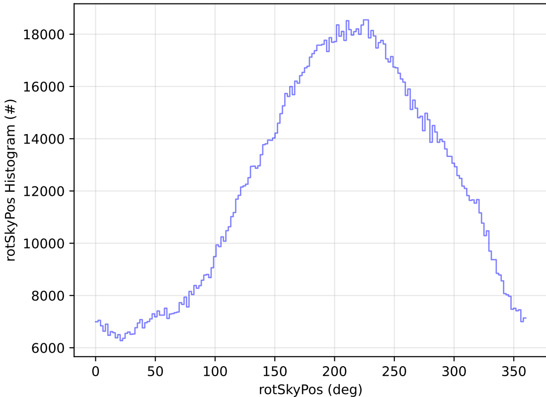
too_elab_r128_d2_griz_v3.4_10yrs WFD all bands: rotSkyPos Histogram
