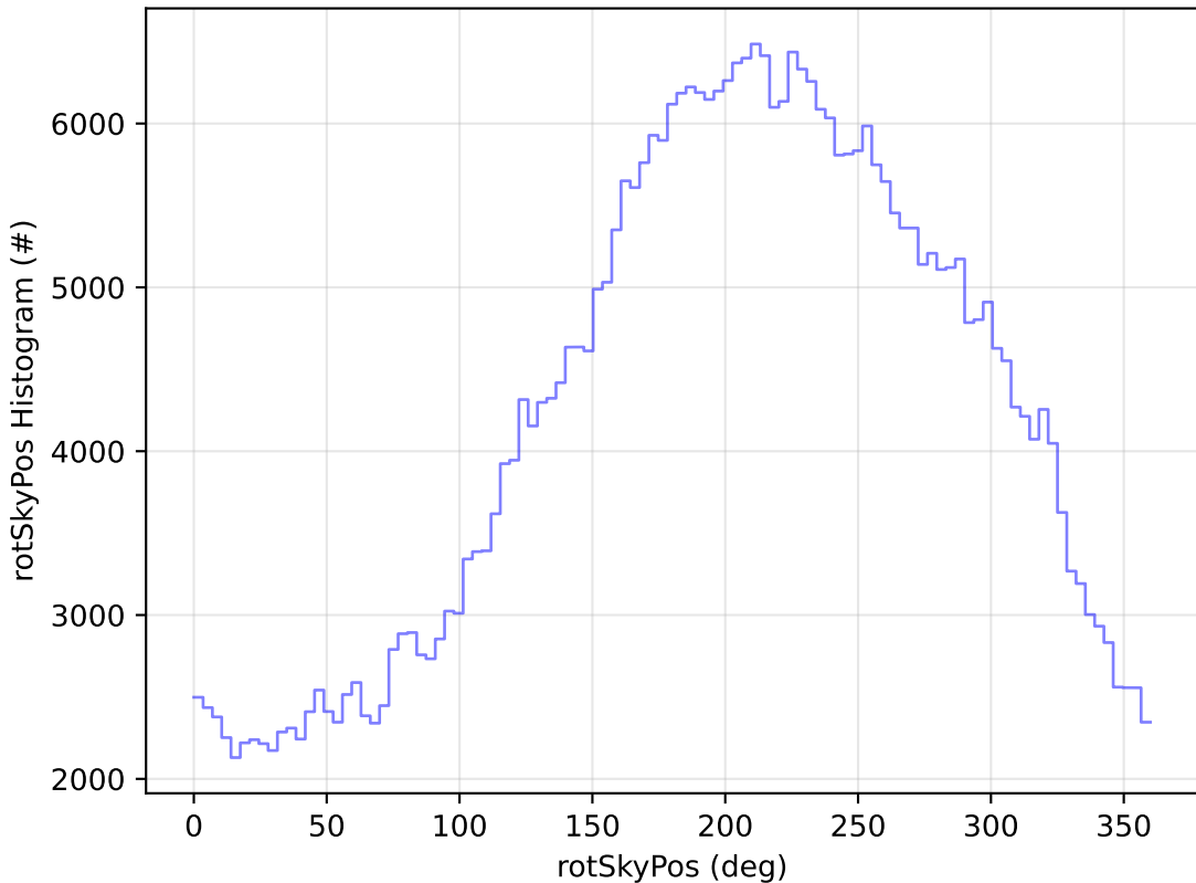
too_elab_r128_d2_griz_v3.4_10yrs All sky z band: rotSkyPos Histogram
