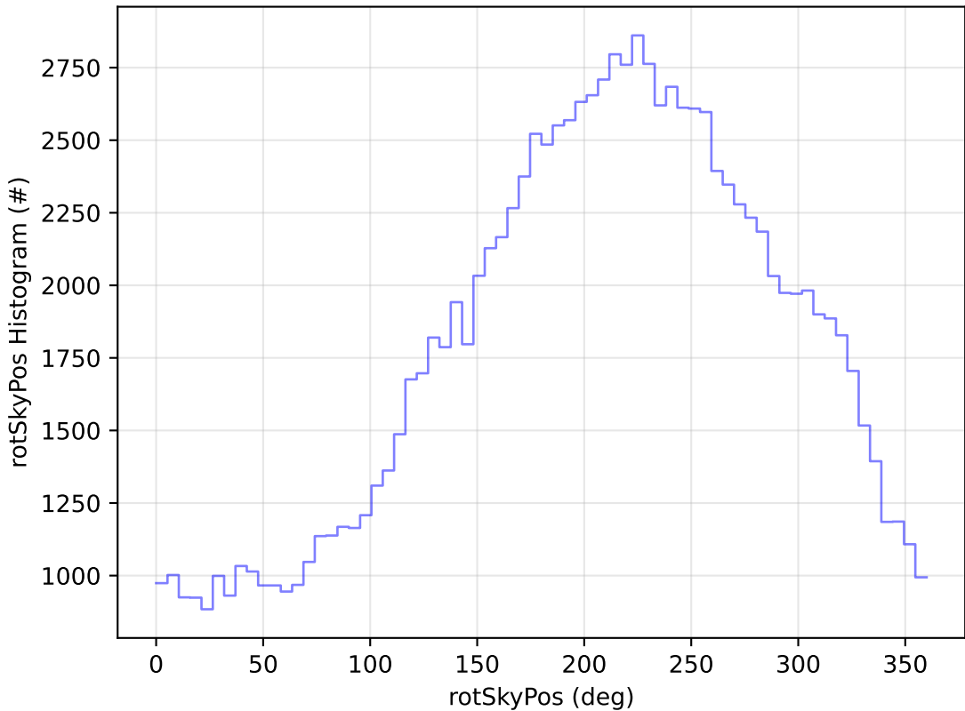
too_elab_r128_d2_griz_v3.4_10yrs All sky u band: rotSkyPos Histogram
