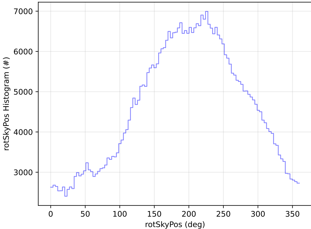
too_elab_r128_d2_griz_v3.4_10yrs All sky r band: rotSkyPos Histogram
