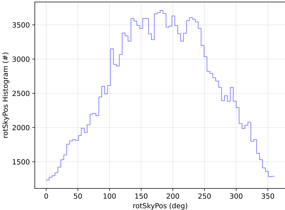
too_elab_r128_d2_griz_v3.4_10yrs All sky g band: rotSkyPos Histogram
