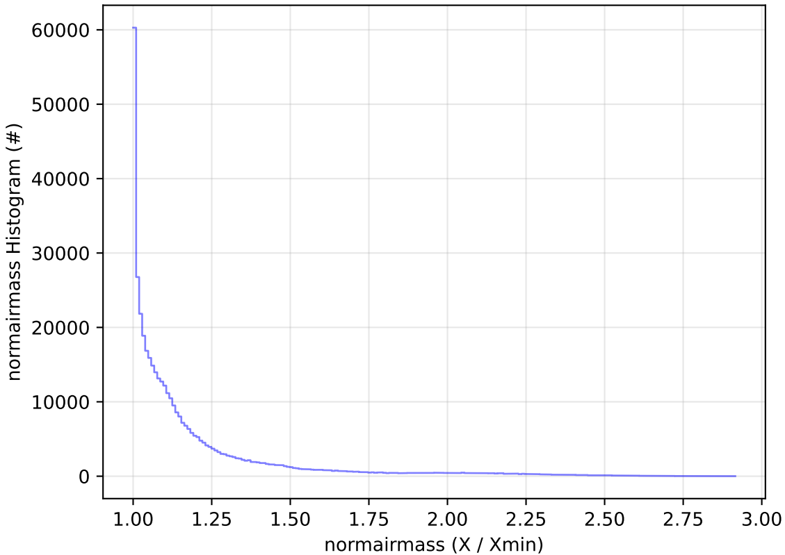
too_elab_r128_d2_griz_v3.4_10yrs WFD z band: normairmass Histogram
