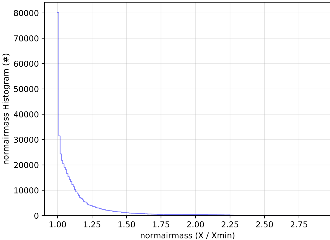
too_elab_r128_d2_griz_v3.4_10yrs WFD r band: normairmass Histogram
