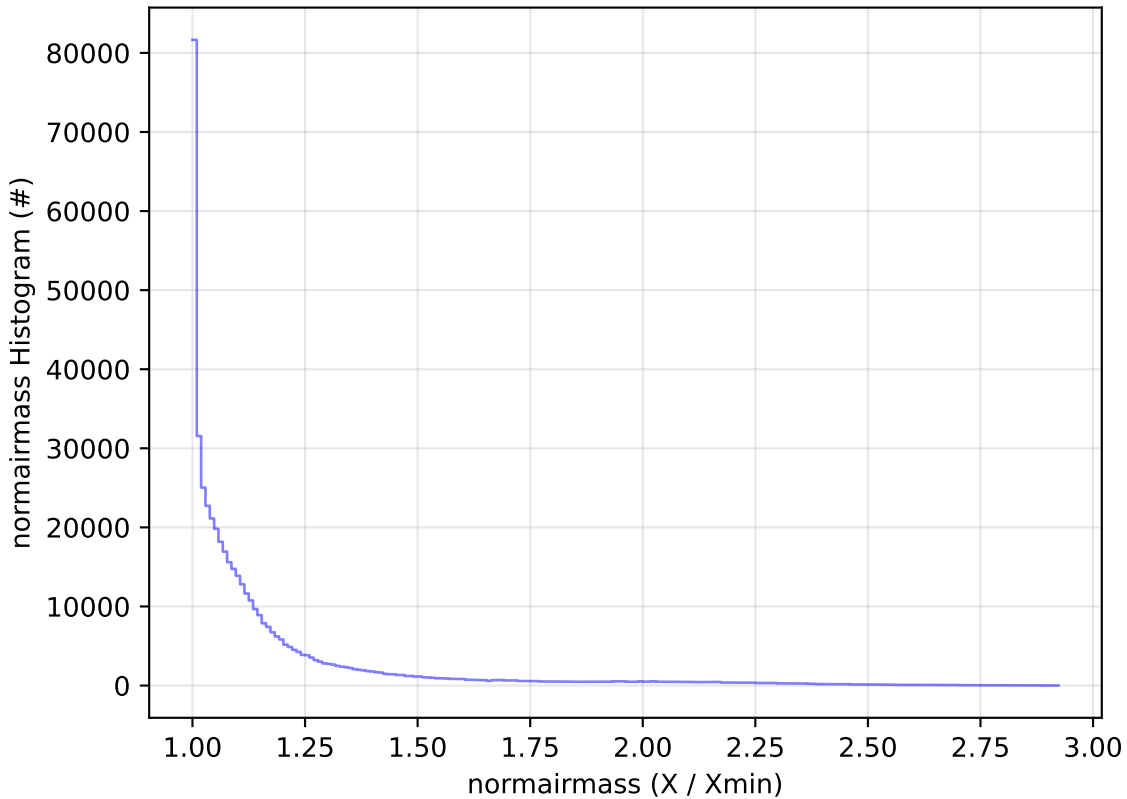
too_elab_r128_d2_griz_v3.4_10yrs WFD i band: normairmass Histogram
