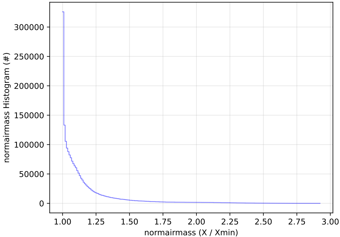
too_elab_r128_d2_griz_v3.4_10yrs WFD all bands: normairmass Histogram
