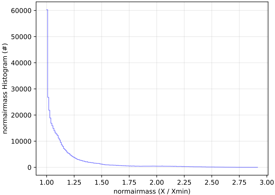
too_elab_r128_d2_griz_v3.4_10yrs All sky z band: normairmass Histogram
