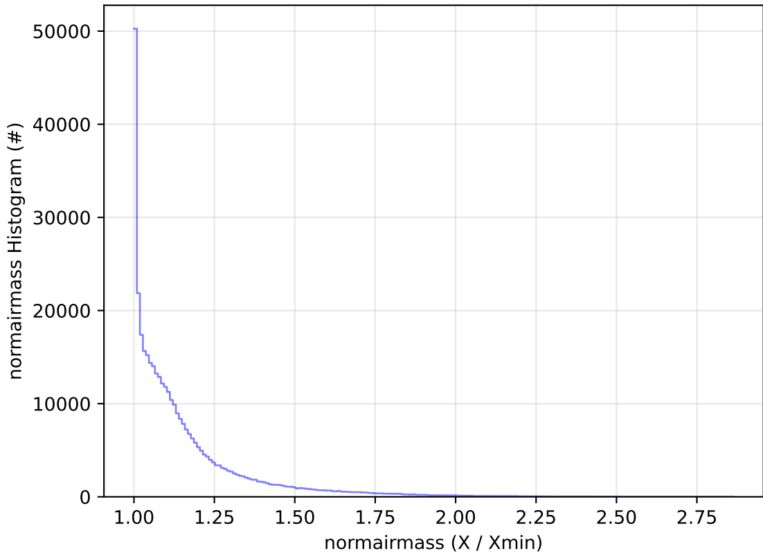
too_elab_r128_d2_griz_v3.4_10yrs All sky y band: normairmass Histogram
