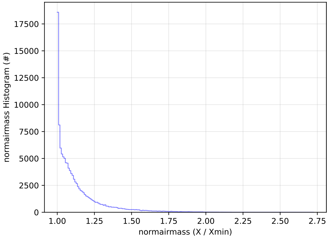
too_elab_r128_d2_griz_v3.4_10yrs All sky u band: normairmass Histogram
