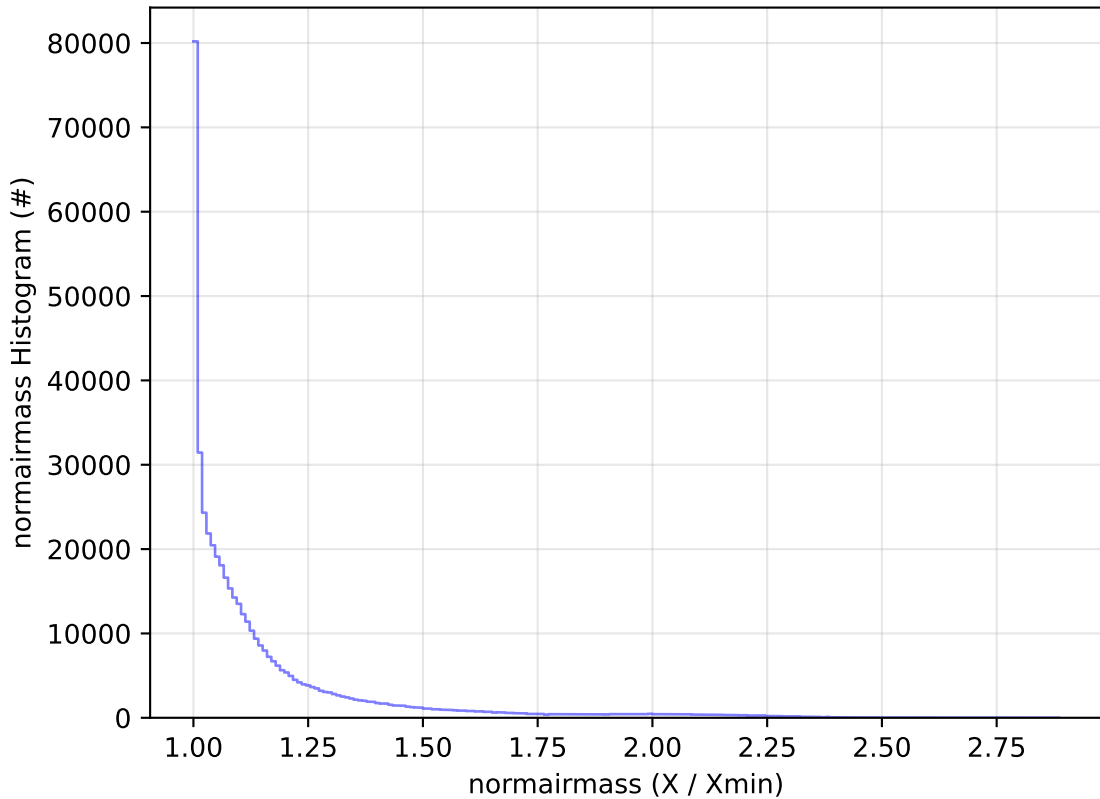
too_elab_r128_d2_griz_v3.4_10yrs All sky r band: normairmass Histogram
