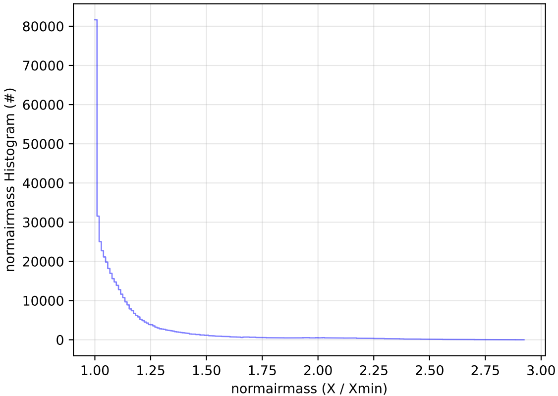
too_elab_r128_d2_griz_v3.4_10yrs All sky i band: normairmass Histogram
