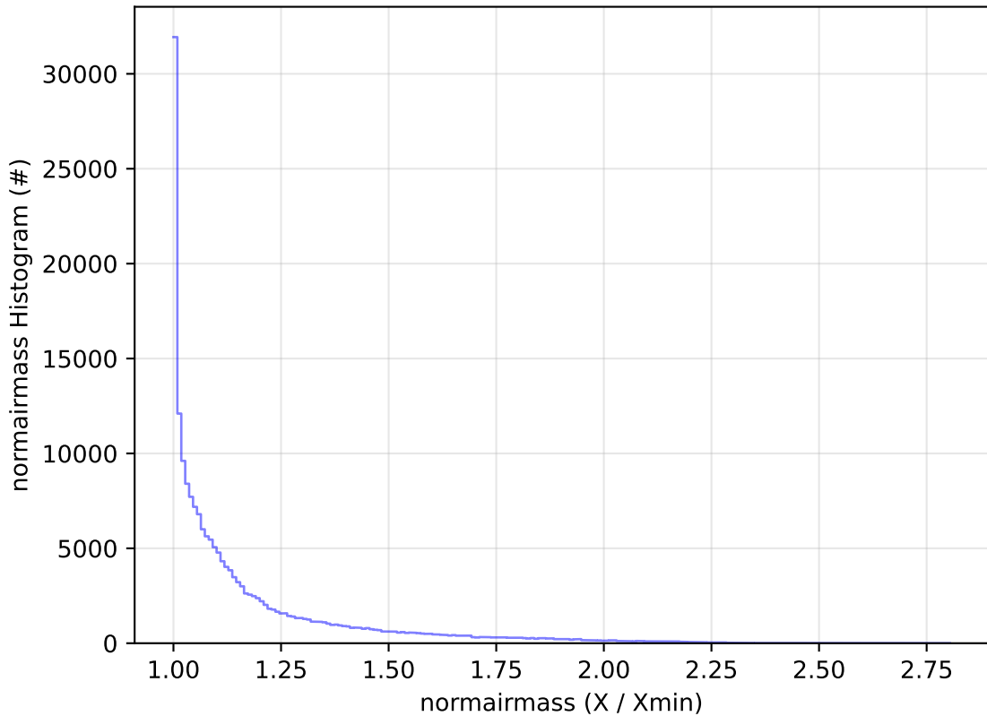
too_elab_r128_d2_griz_v3.4_10yrs All sky g band: normairmass Histogram
