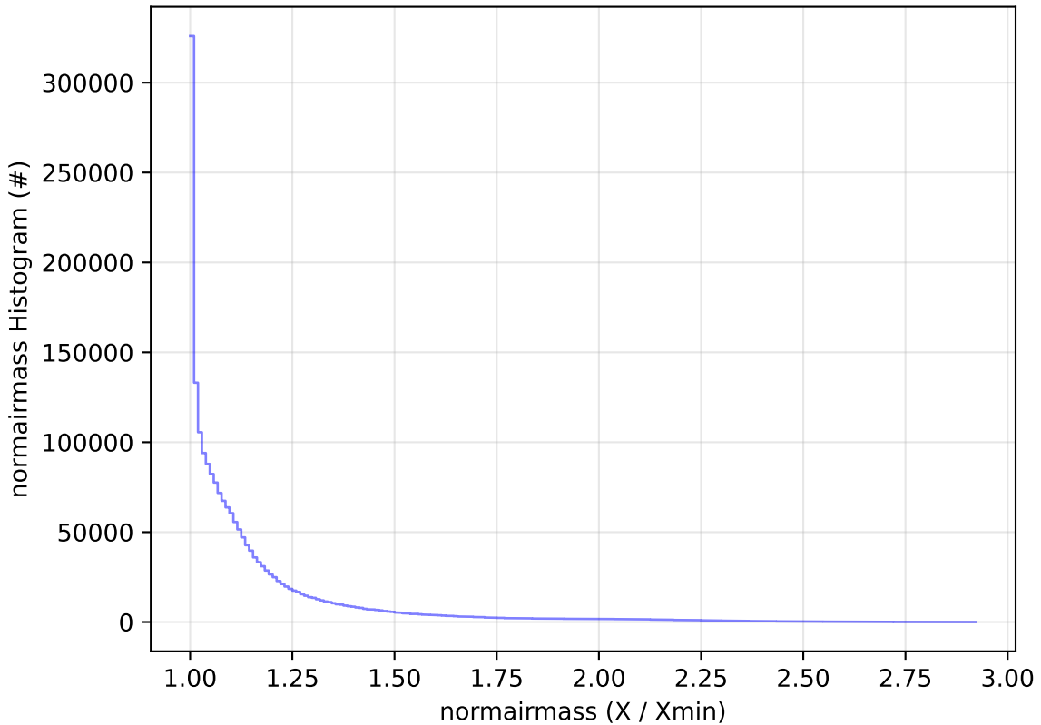
too_elab_r128_d2_griz_v3.4_10yrs All sky all bands: normairmass Histogram
