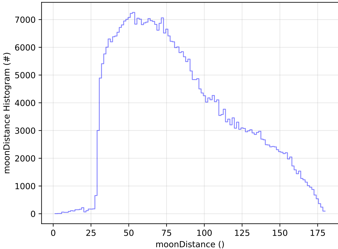
too_elab_r128_d2_griz_v3.4_10yrs WFD z band: moonDistance Histogram
