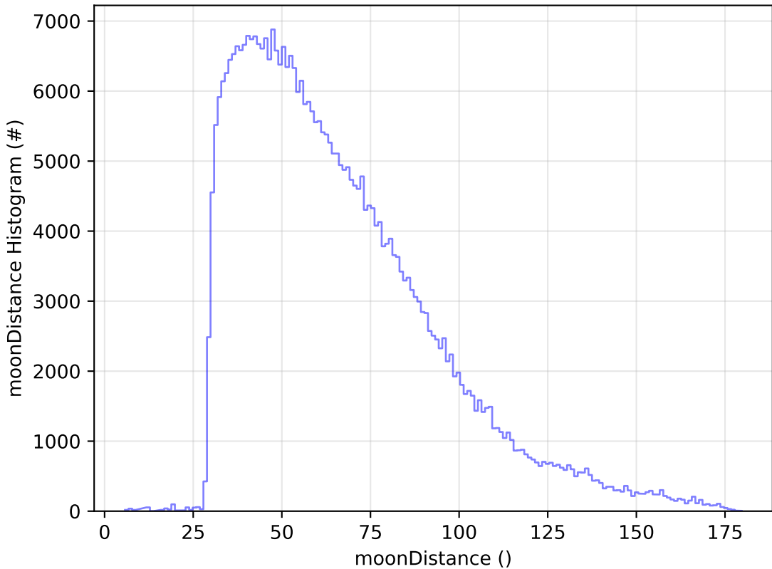
too_elab_r128_d2_griz_v3.4_10yrs WFD y band: moonDistance Histogram
