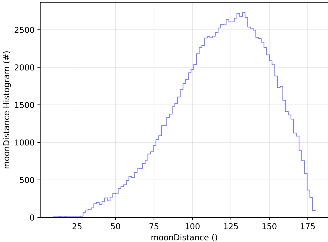
too_elab_r128_d2_griz_v3.4_10yrs WFD u band: moonDistance Histogram
