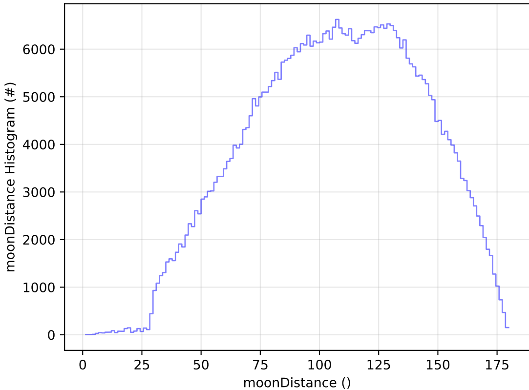
too_elab_r128_d2_griz_v3.4_10yrs WFD r band: moonDistance Histogram
