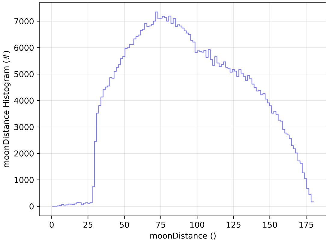
too_elab_r128_d2_griz_v3.4_10yrs WFD i band: moonDistance Histogram
