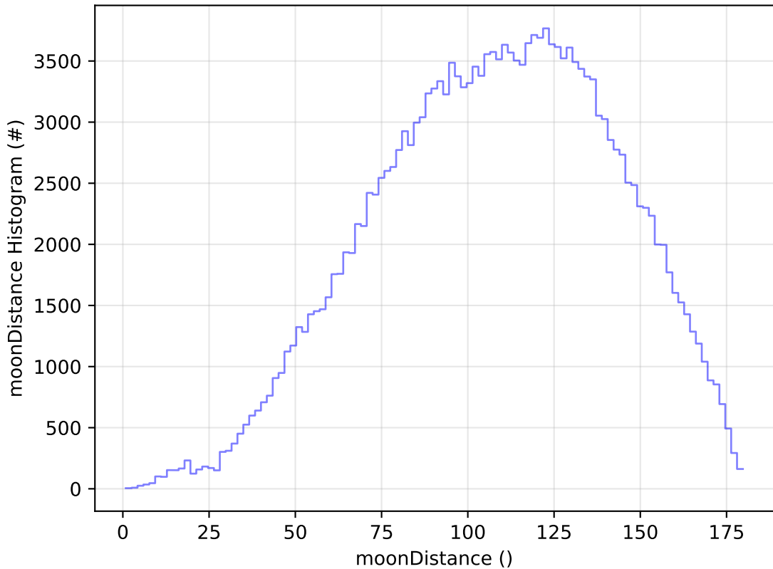
too_elab_r128_d2_griz_v3.4_10yrs WFD g band: moonDistance Histogram
