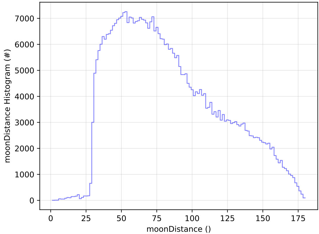
too_elab_r128_d2_griz_v3.4_10yrs All sky z band: moonDistance Histogram
