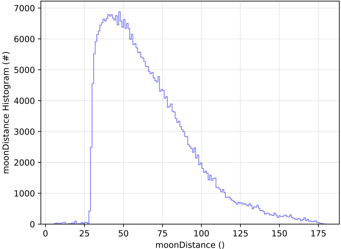
too_elab_r128_d2_griz_v3.4_10yrs All sky y band: moonDistance Histogram
