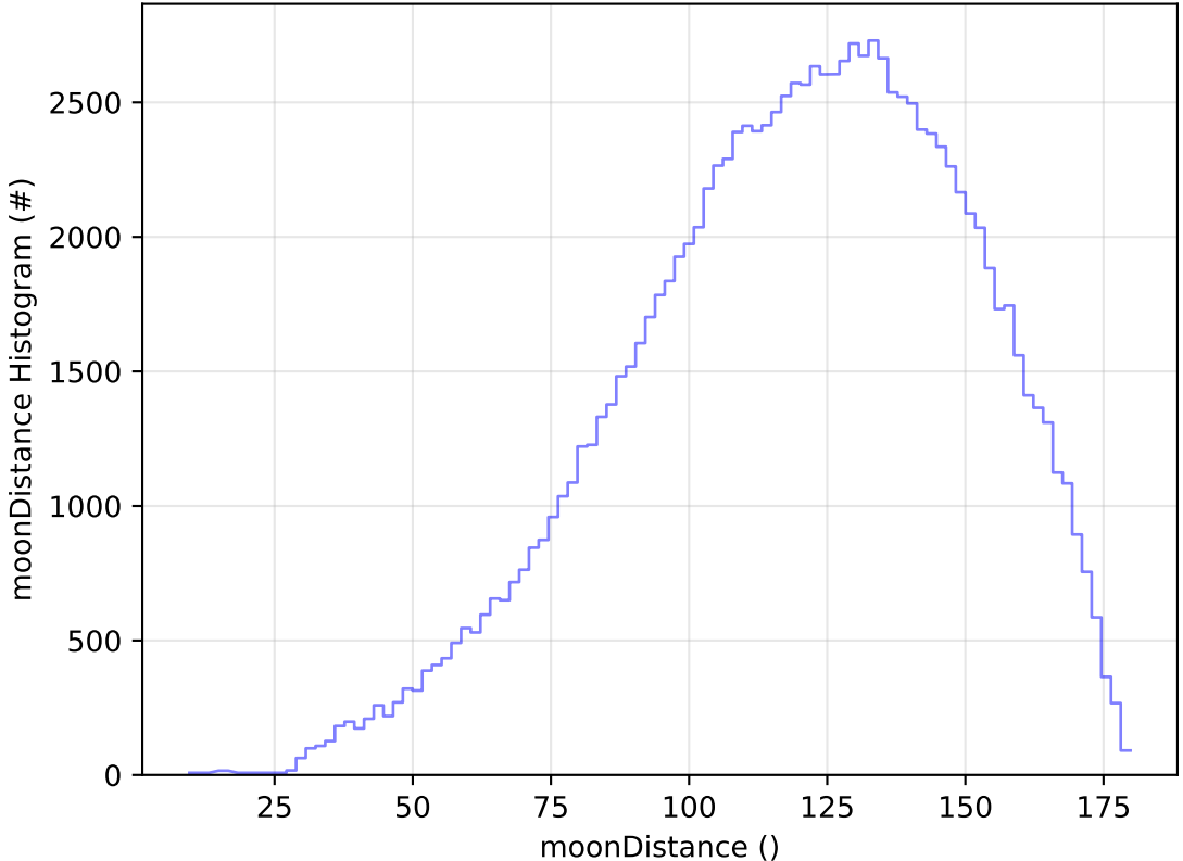
too_elab_r128_d2_griz_v3.4_10yrs All sky u band: moonDistance Histogram
