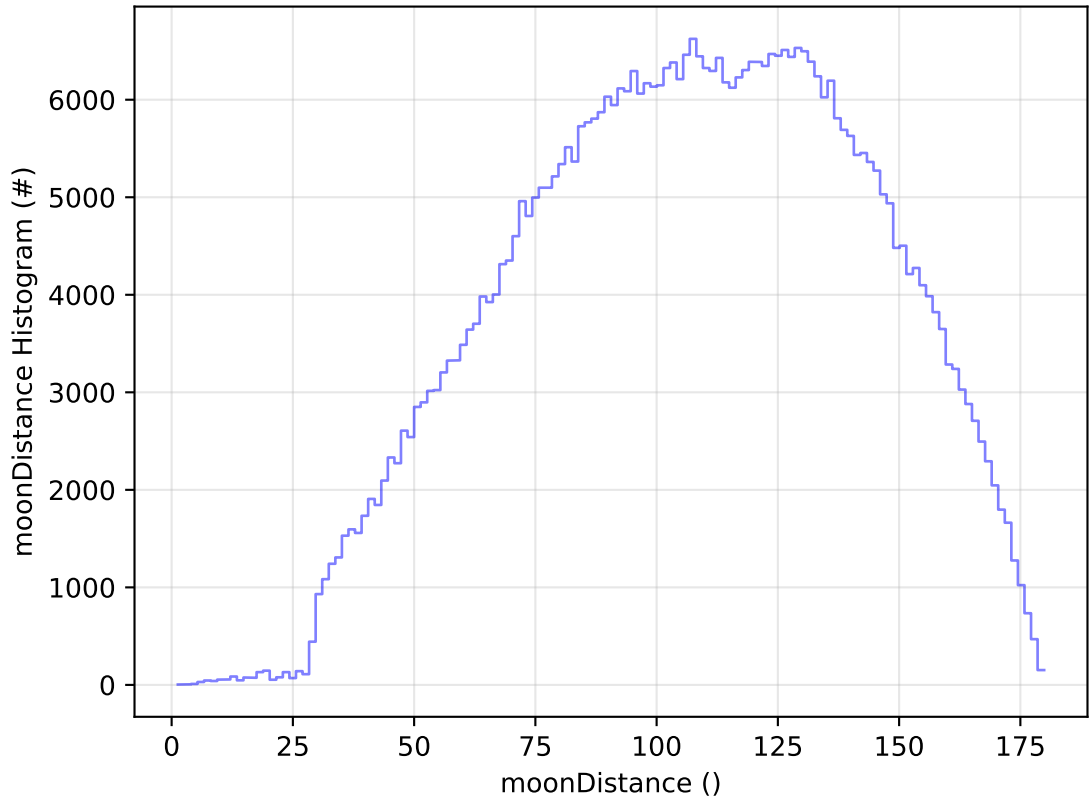
too_elab_r128_d2_griz_v3.4_10yrs All sky r band: moonDistance Histogram
