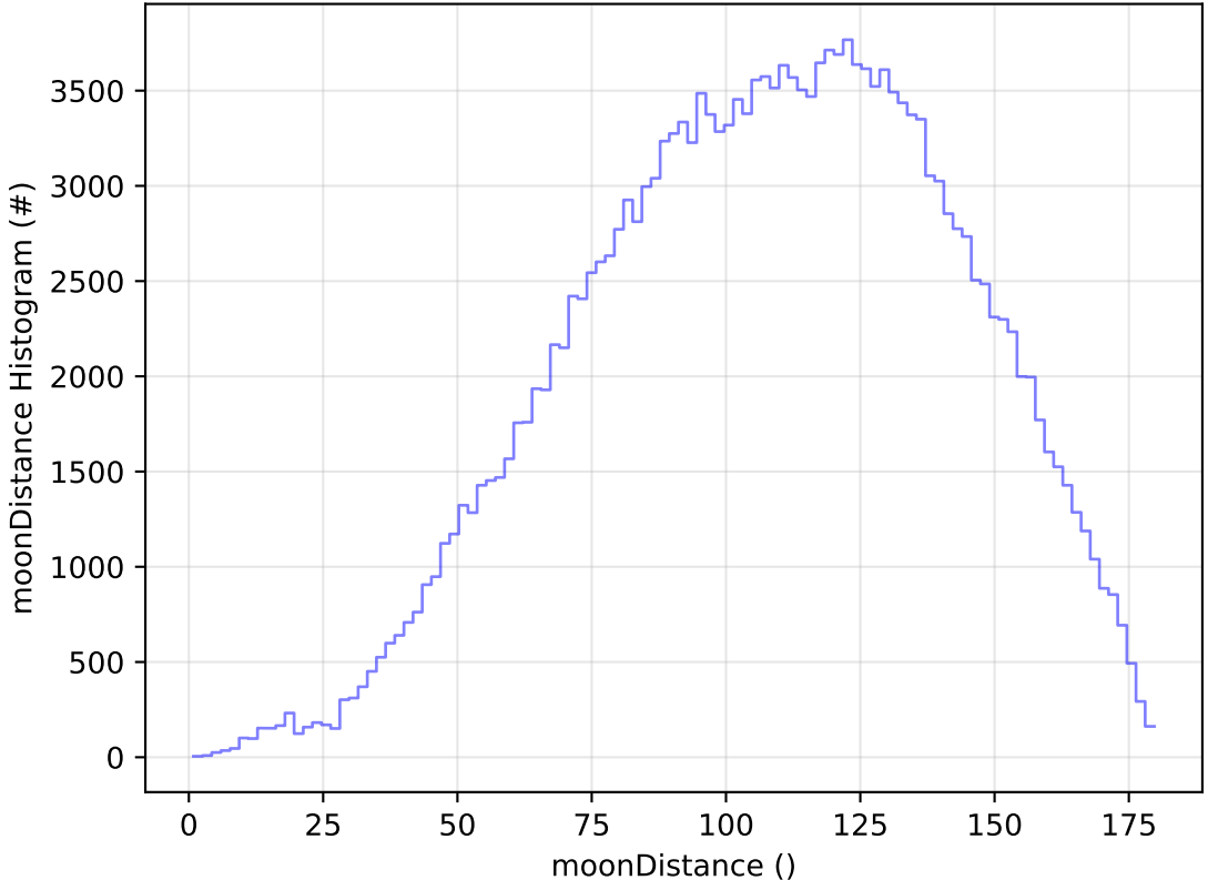
too_elab_r128_d2_griz_v3.4_10yrs All sky g band: moonDistance Histogram
