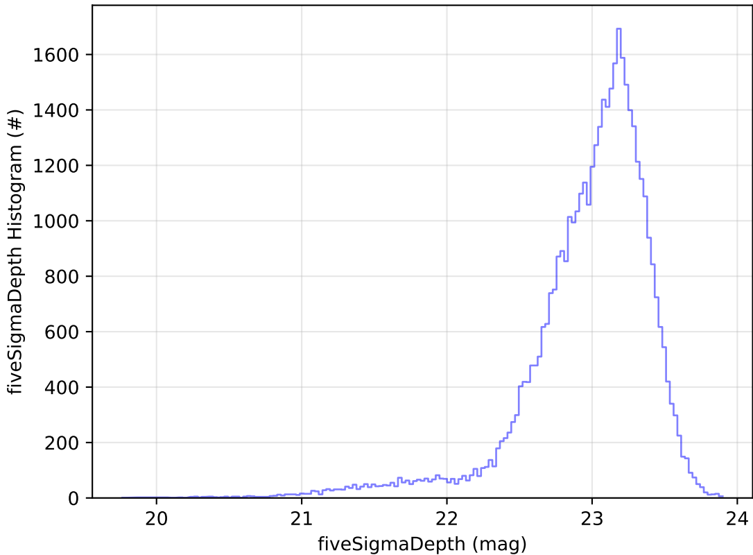
too_elab_r128_d2_griz_v3.4_10yrs Yr 1 z band: fiveSigmaDepth Histogram
