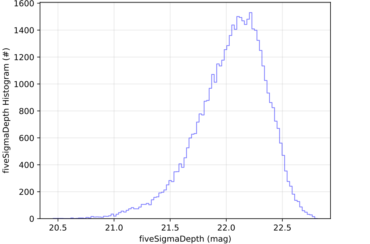
too_elab_r128_d2_griz_v3.4_10yrs Yr 1 y band: fiveSigmaDepth Histogram
