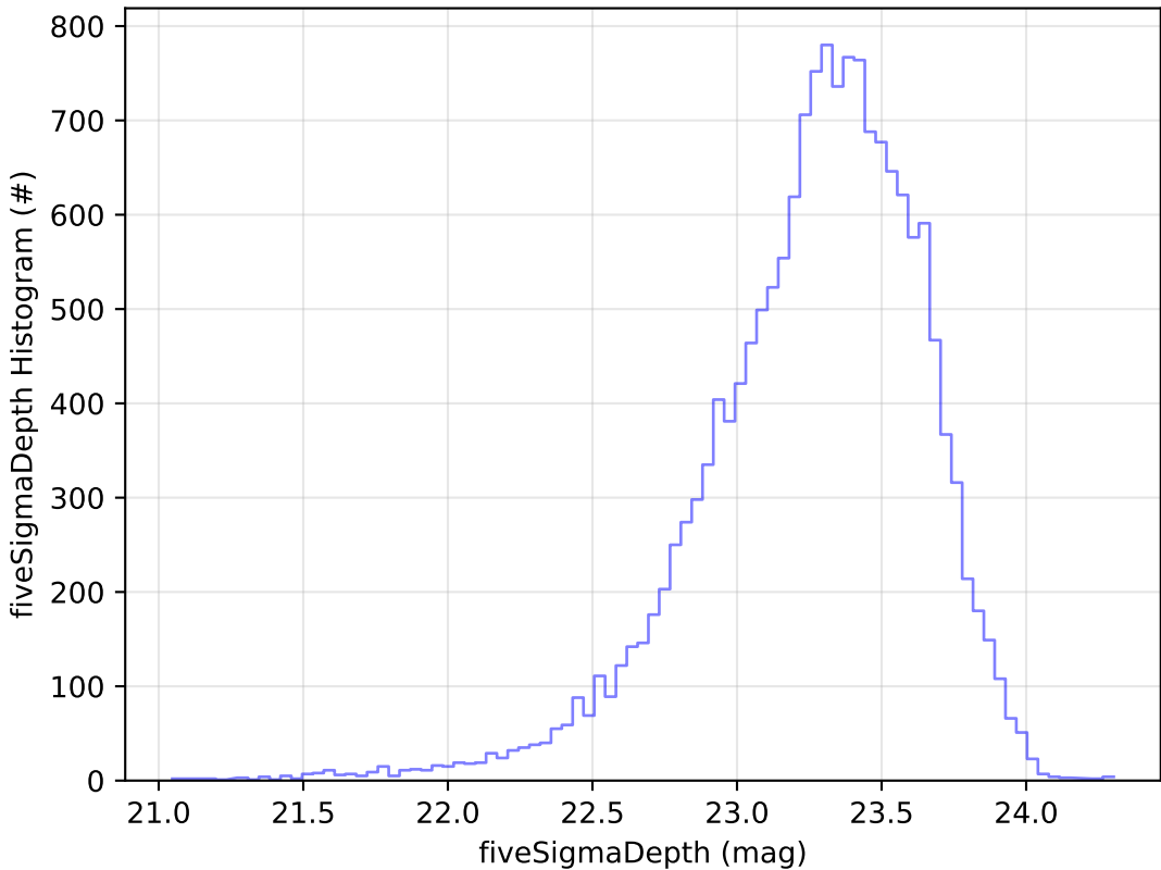
too_elab_r128_d2_griz_v3.4_10yrs Yr 1 u band: fiveSigmaDepth Histogram
