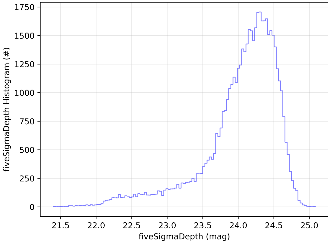
too_elab_r128_d2_griz_v3.4_10yrs Yr 1 r band: fiveSigmaDepth Histogram
