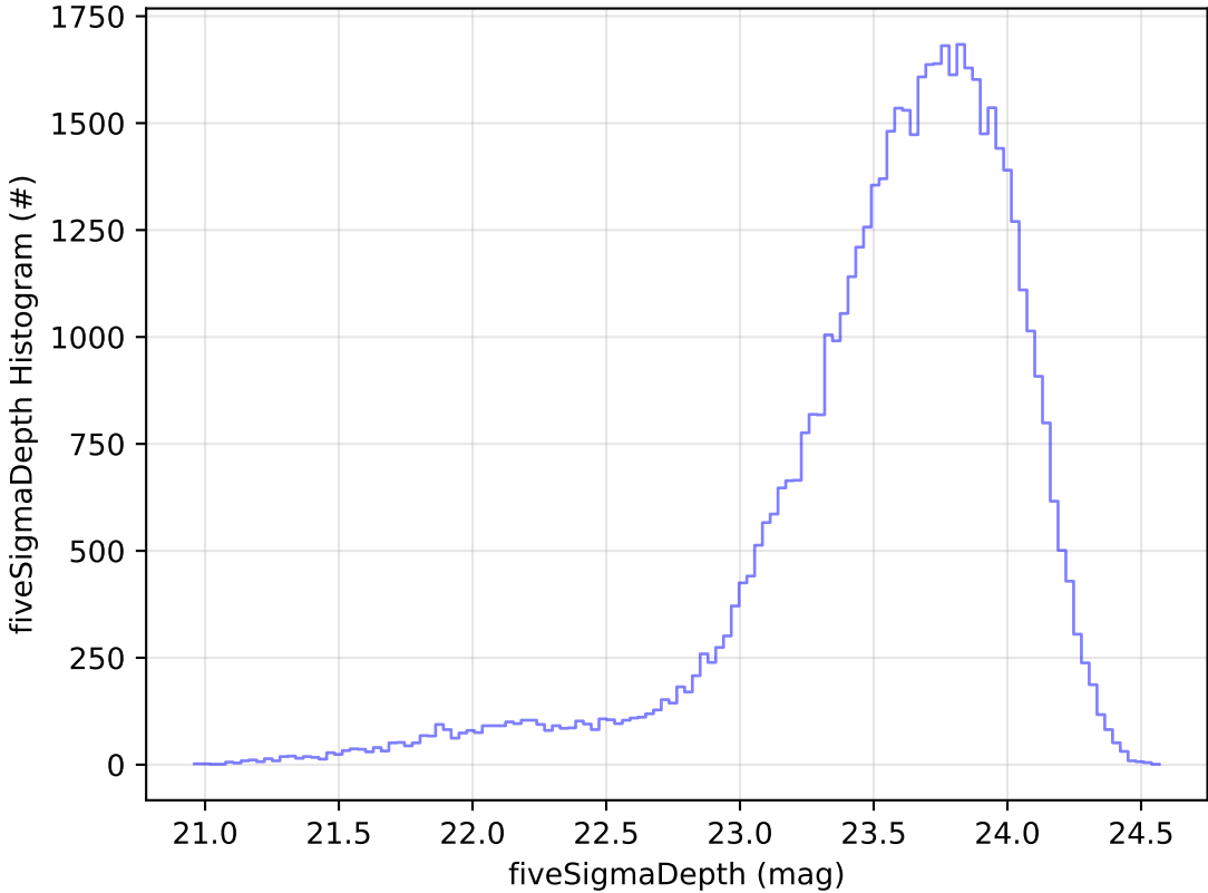
too_elab_r128_d2_griz_v3.4_10yrs Yr 1 i band: fiveSigmaDepth Histogram
